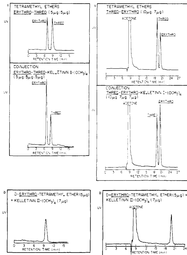
Figure 4. HPLC coelution of (a) kellestinin I tetramethyl ether and synthetic 1b (erythro) and (b) kellestinin II tetramethyl ether and synthetic 2b . Conditions: Waters Associates HPLC; 260-nm UV detector; flow rate 1.5 mL/min. Left: 25 cm × 4.6 mm Chromanetics LiChrosorb SI-60 column; mobile phase methanol-dichloromethane (0.25:99.75). Right: 25 cm × 10 mm Altex Ultrasphere-ODS column; mobile phase methanol-water (90:10).
