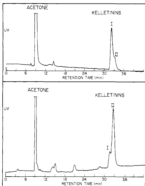
Figure 1. HPLC analysis of silica column fractions enriched in kelletinins I (top) or II (bottom). Conditions: Waters Associates HPLC; 260-nm UV detector; 25 cm × 10 mm Altex Ultrasphere-ODS column; mobile phase methanol-water (65:35); 0.1 N NaOAc/HOAc to pH 4.6; flow rate 1.5 mL/min.
