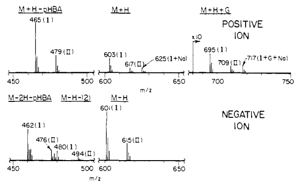
Figure 2. Fast atom bombardment (FAB) mass spectra (partial) of kelletinins I and II (mixture).
