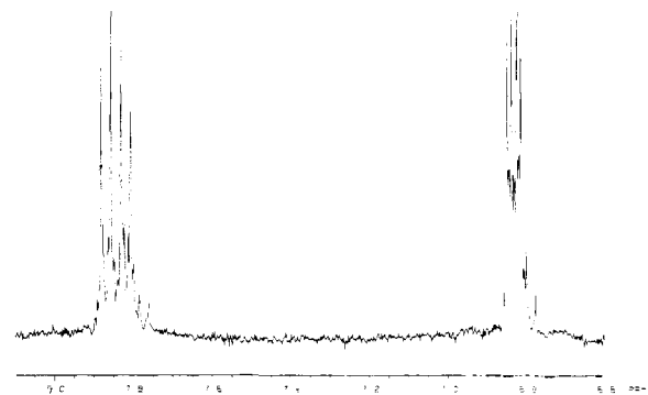
Figure 3. 1 H NMR spectrum (CD 3 CN) of kelletinins I in the aromatic region.
